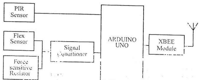
Fig 2. Transmitting section
